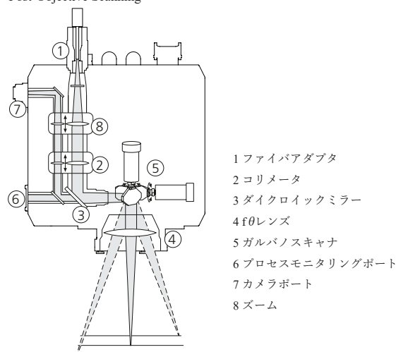
Post-Objective Scanning
