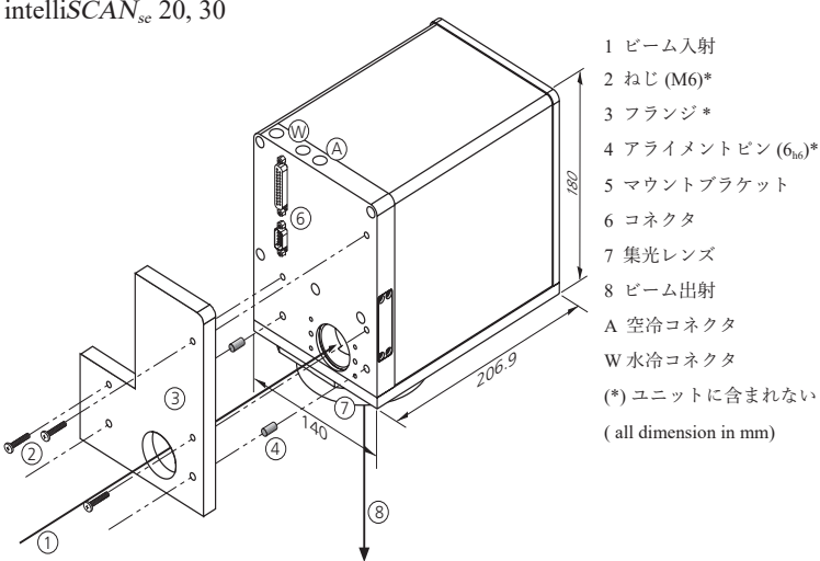
intelliSCAN sc 20, 30
